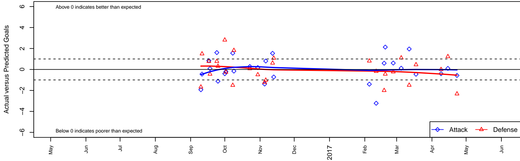
LYS Red B06 Dots are actual minus expected GF (blue circles) and GA (red triangles). Blue line is smoothed change in attack strength. Red is smoothed change in defense strength.
